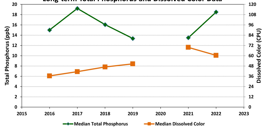
Figure 5. Belleau Lake - Deep Site (2016-2022) Long-term Total Phosphorus and Dissolved Color Data
