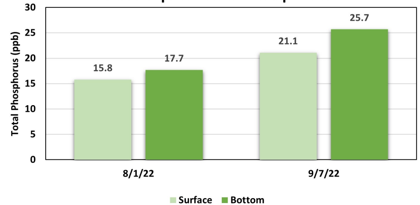
Figure 9. Belleau Lake - Site 1 Deep Total Phosphorus inter-comparison
