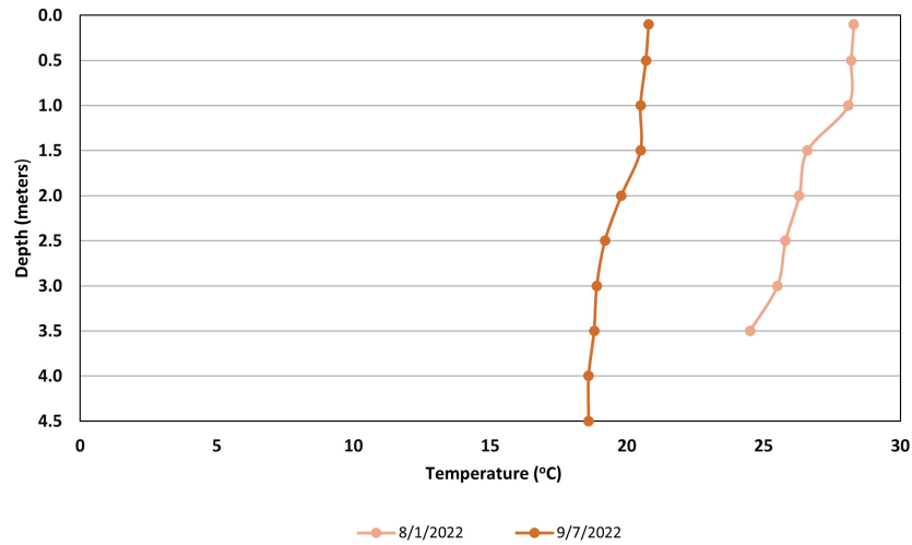
Figure 6. Belleau Lake - Site 1 Deep Temperature Profiles (August 1 through September 7, 2022)
