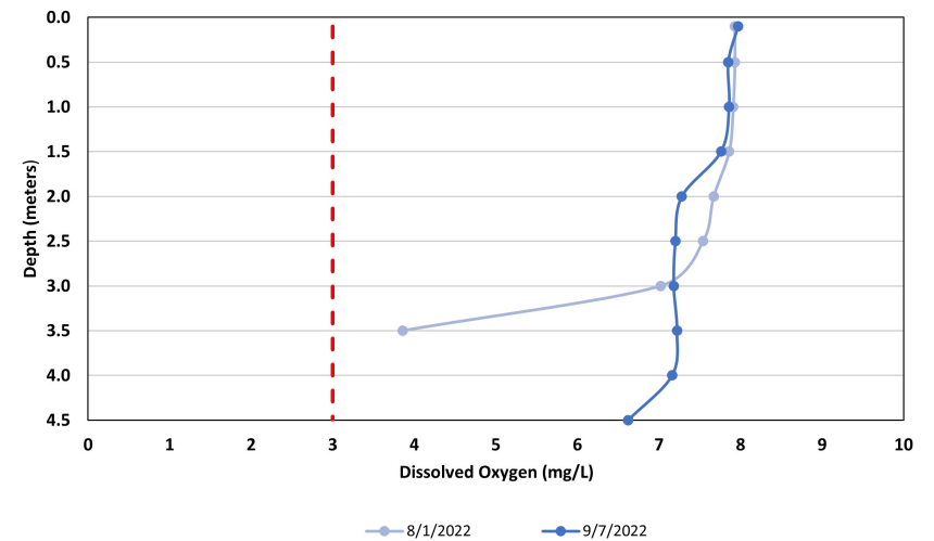
Figure 7. Belleau Lake - Site 1 Deep Dissolved Oxygen Profiles (August 1 through September 7, 2022)
