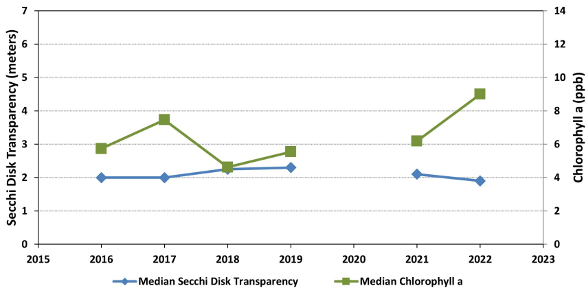
Figure 4. Belleau Lake - Deep Site (2016-2022) Long-term Secchi Disk Transparency and Chlorophyll a Data
