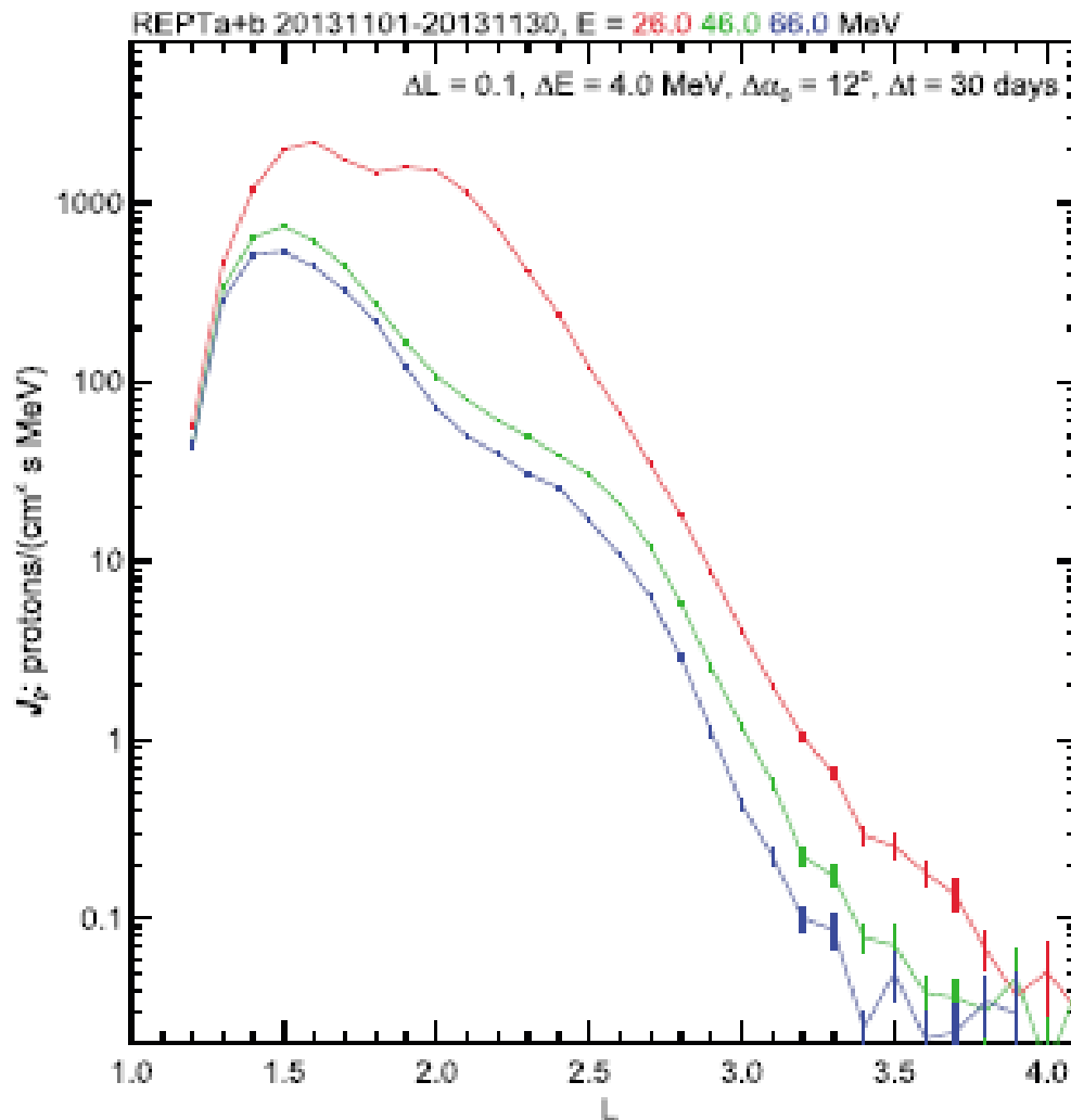
Figure 2.5: The above figure shows measured average equatorial differential omnidirectional proton intensity as a function of geomagnetic shells L. Three proton energies are represented in red (26 MeV), green (46 MeV) and blue (66 MeV). [5]
