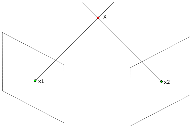
Figure 5.2: Triangulation
