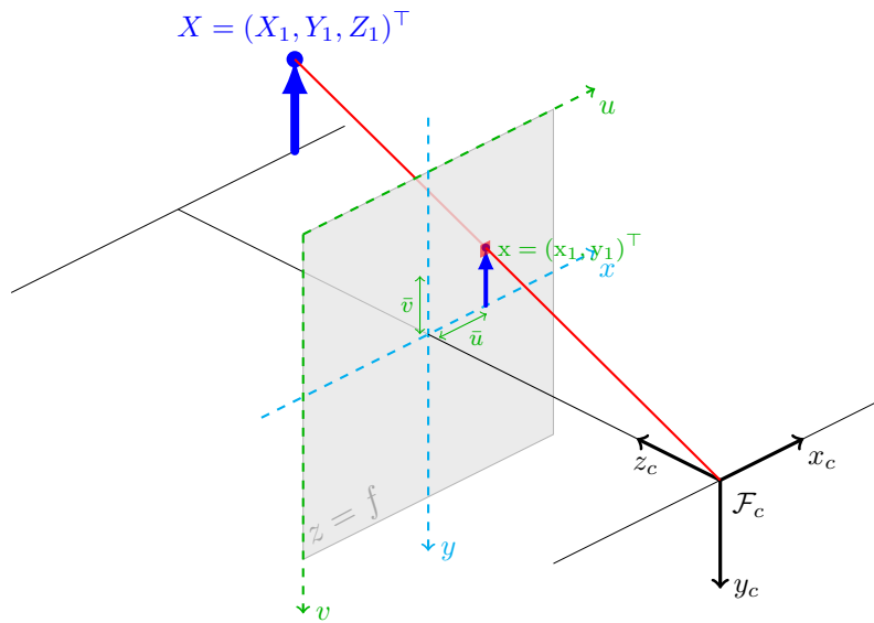
Figure 2.1: Pinhole camera model
