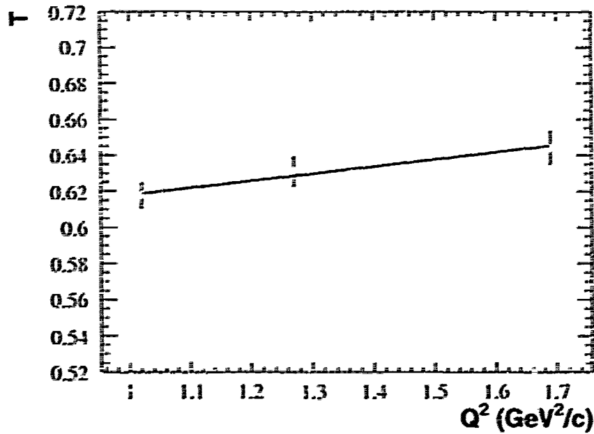
Figure 6-10. The Nuclear Transparency ratio for Carbon and Deuterium targets with beam energy of 5\text{GeV} is plotted here as a function of Q^2 . The error bars in each point show the different contribution from statistical error (black) and systematic point to point error (red). The data is fitted with a linear function (black line). The result of the fit gives for the slope for the Nuclear Transparency as a function of Q^2 a value of (0.039 \pm 0.017_{stat} \pm 0.034_{sys})\text{GeV}^{-2}
