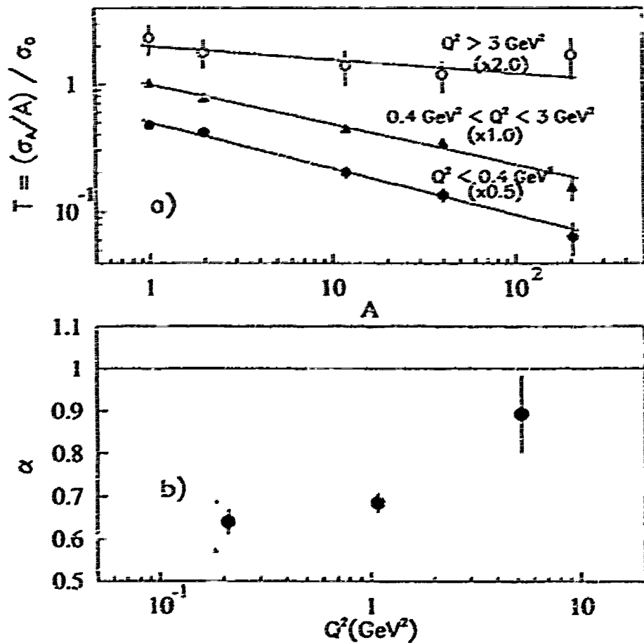
Figure 1-18 The Transparencies T = \sigma_A / A\sigma_0 (where \sigma_A = \sigma_0 A^\alpha ) for the experiment E665 at Fermilab [15]. Here the data respectively of \rho^0 electroproduction off hydrogen, deuterium, Carbon, Calcium and Lead is plotted versus A for three different bins in Q^2 . The three sets of points have been multiplied by \times 2.0 ( Q^2 > 3 \text{ GeV}^2 ), \times 1.0 ( 0.4 \text{ GeV}^2 < Q^2 < 3 \text{ GeV}^2 ), \times 0.5 ( Q^2 < 0.4 \text{ GeV}^2 ). The \alpha found in the fit is then plotted in the lower picture as a function of Q^2 (A value of \alpha = 1 will indicate full transparency). Color Transparency will imply a Q^2 dependence for the parameter \alpha in kinematical range of this experiment. The error here are just statistical.
