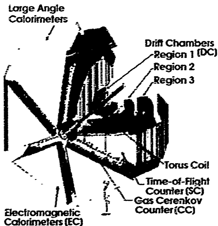
Figure 2-3: The CLAS detector and its components
