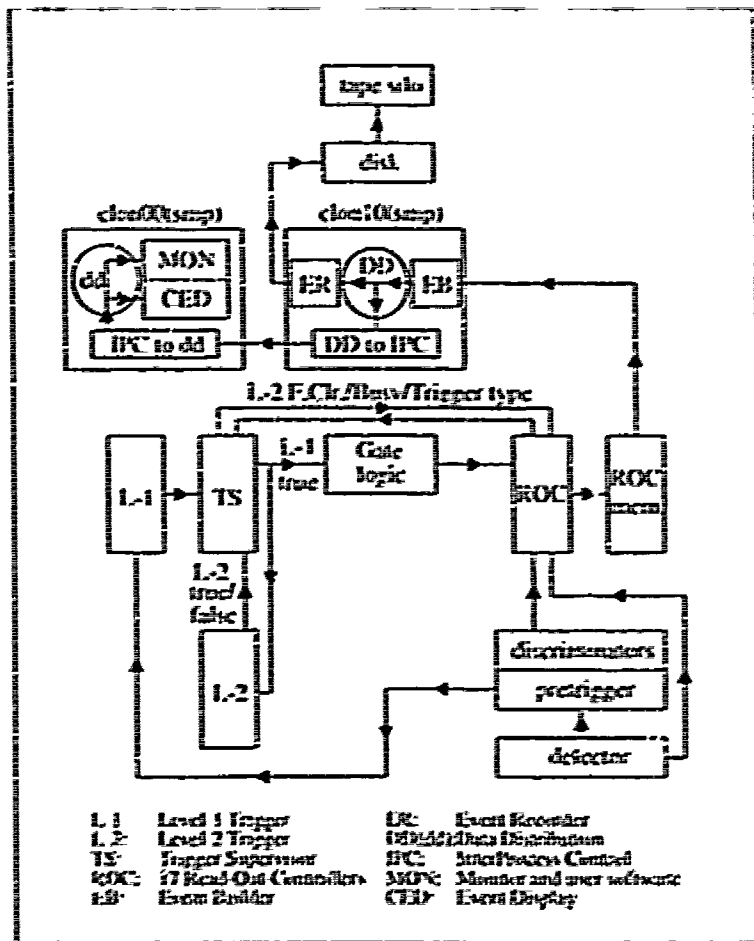
Figure 2-19: Schematic Diagram for the Data Acquisition system
