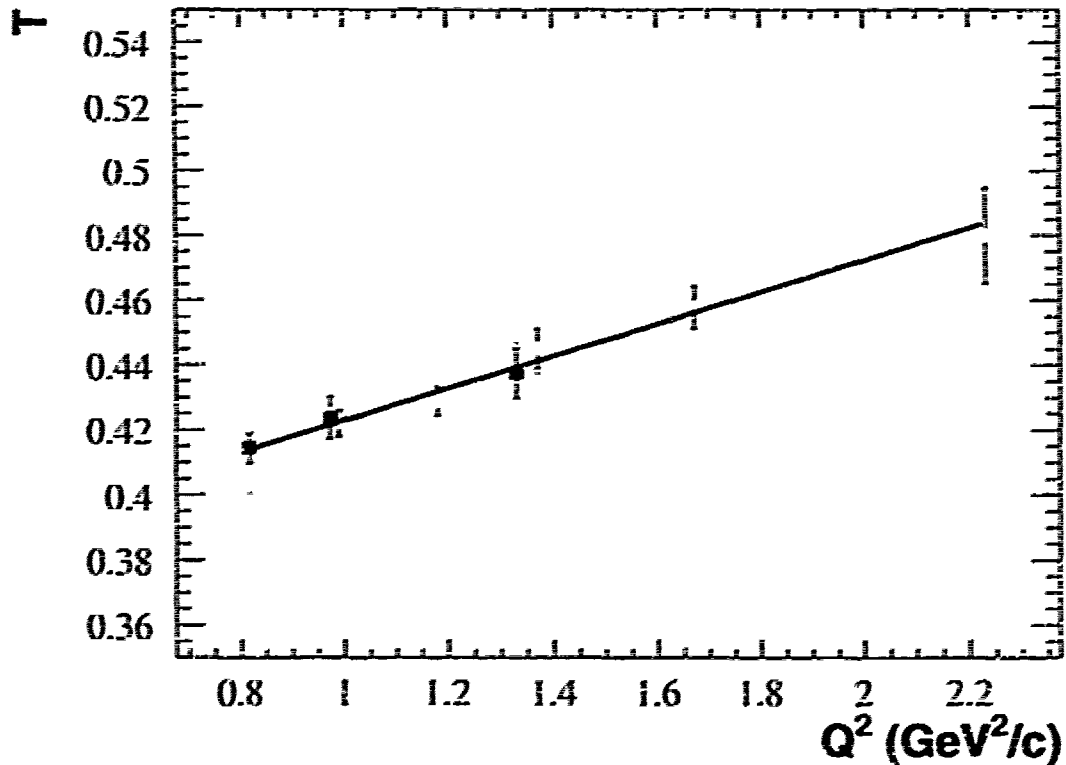
Figure 6-11. The Nuclear Transparency ratio for Iron and Deuterium targets with beam energy of 4GeV (blue) and 5GeV (green) is plotted here as a function of Q^2 . The error bars in each point show the different contribution from statistical error (black) and systematic point to point error (red). The data is fitted with a linear function (black line). The result of the fit gives for the slope for the Nuclear Transparency as a function of Q^2 a value of (0.0195 \pm 0.0069_{stat} \pm 0.0124_{syst})GeV^{-2}
