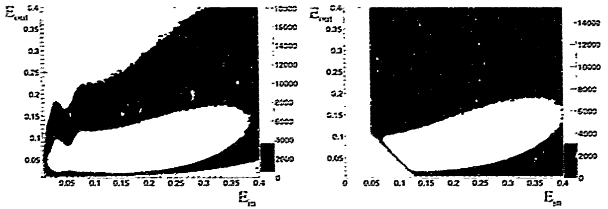
Figure 3-3: E_{out} vs E_{in} plot before (left) and after (right) EC cut
