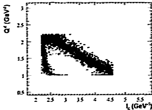
Figure 6-1: The l_c vs Q^2 distribution is shown here for the Iron target. At first we will consider the region in the shadow, characterized by 1.9\text{GeV}^2 < Q^2 < 1.6\text{GeV}^2 . In this region we will determine the experimental transparency ratio dependence on l_c (see figure 6-2 on the right)
