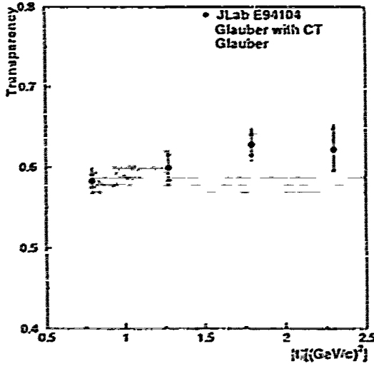
Figure 1-14: Nuclear Transparency for {}^4\text{He} [14] as a function of the momentum transfer square |t| for \theta_{cm} = 70^\circ . Theoretical prediction of a Glauber model calculation and a Glauber model with CT are also shown.
