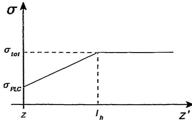
Figure 1-11. Cross section evolution in space from the creation of a Point Like Configuration ( \sigma_{PLC} ) to the creation of the final vector meson as described in equation 1.40
