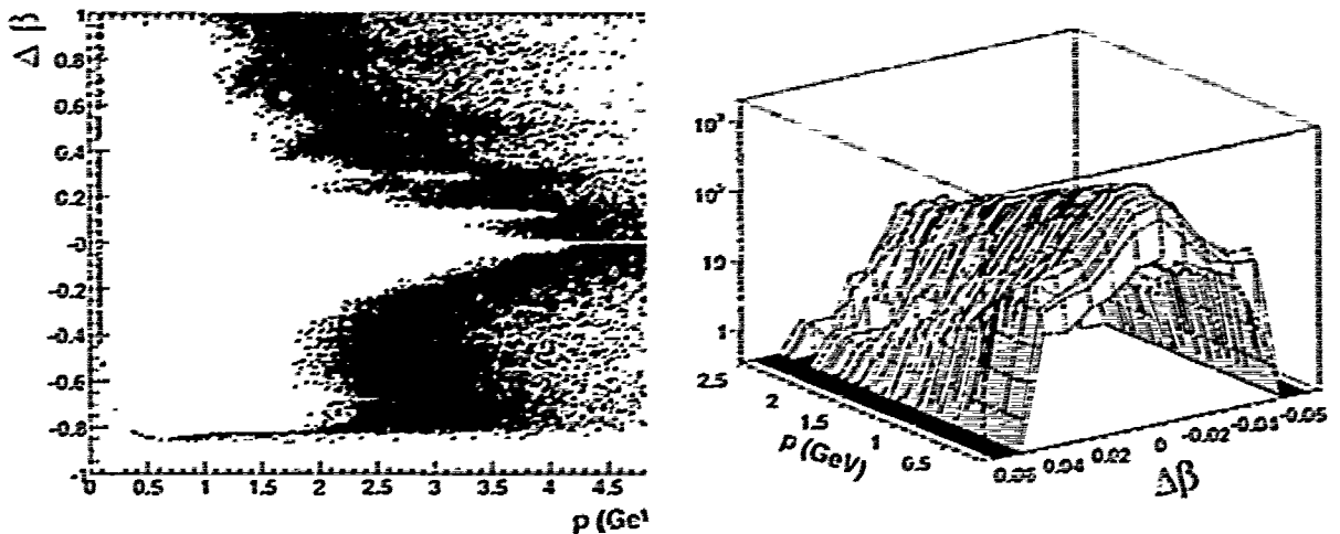
Figure 3-6. \Delta\beta is plotted here as a function of the track's momentum p express in GeV . A cut has been placed around the x axis ( |\Delta\beta| < 0.05 ). The result of the cut shown in the picture on the right. The points at |\Delta\beta| = 0.05 represent the \pm 2\sigma cut for the distribution determined at constant momentum and centered around |\Delta\beta| = 0
