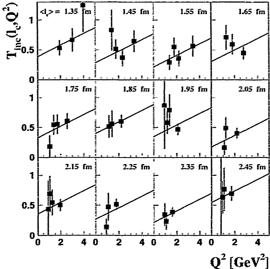
Figure 1-21. Nuclear Transparency as a function of Q^2 in different coherence length bins of 0.1 \text{ fm} for incoherent p^0 electroproduction on Nitrogen [19]. A fit T_A = P_0 + P_1 Q^2 was used in each l_c bin, the parameter P_1 being common to all the bins. This permitted a better definition of the slope of the Transparency vs Q^2 , phenomena that is due to Color Transparency. The slope was found to be P_1 = (0.689 \pm 0.046 \pm 0.020) \text{ GeV}^{-2}
