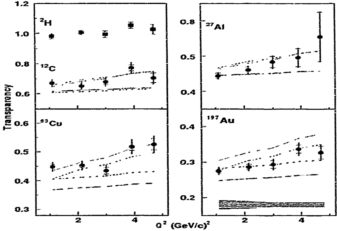
Figure 1-16. Nuclear Transparency T is defined as (\frac{Y}{Y_{MC}})_A / (\frac{Y}{Y_{MC}})_H vs Q^2 for different target combinations[15]. The model used for interpreting the data are: Glauber model (solid red line). Glauber model + CT (dashed red line). Glauber model including Short Range Correlations (blue dot-dash line). Glauber model including SRC + CT (blue dotted line). The dark band in the bottom right panel represents the model uncertainties and is common to all targets.
