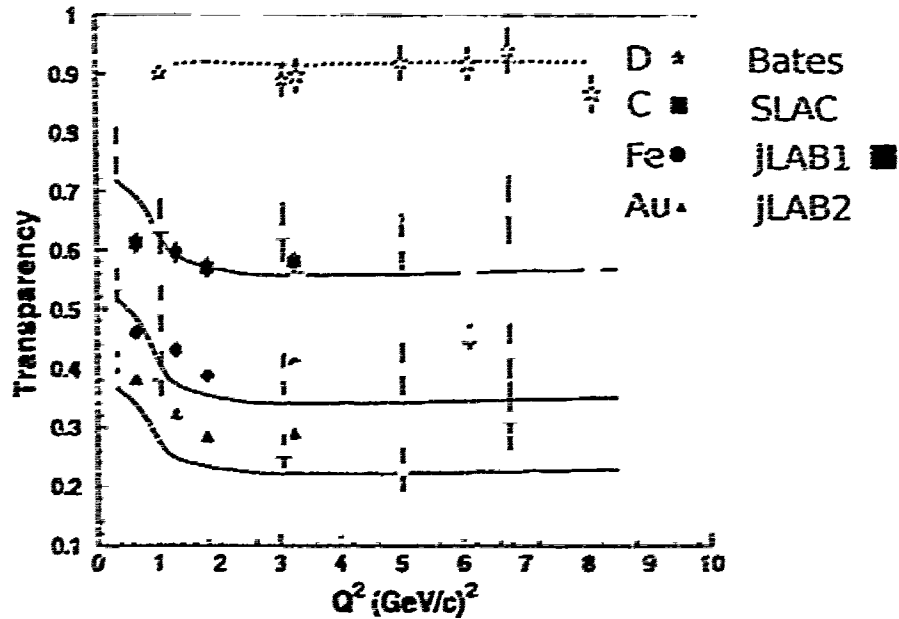
Figure 1-13. The quasi-free e, e', p reaction has been studied at several facilities with a Q^2 range of 0 - 9(GeV/c) 2 . Here are the results from Bates (for this experiment the data points refer from top to bottom respectively to Carbon, Nickel and Tantalum), [7], from SLAC [8] [9] and from Jefferson Lab ([10] (1)) ([11] (2)). The theoretical curves using Glauber calculations (solid curves from [12], dashed curve from [13]) predicts the experimental behavior well, indicating that all these experiments lack the expected increase due to Color Transparency
