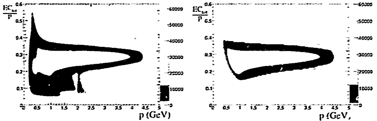
Figure 3-4: \frac{EC_{out}}{p} vs p plot before (left) and after (right) 3\sigma cut
