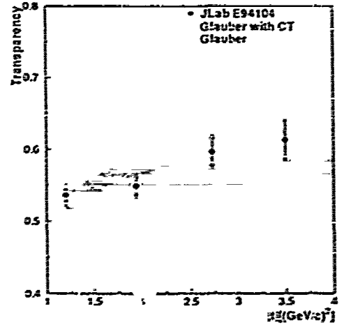
Figure 1-15: Nuclear Transparency for {}^4\text{He} [14] as a function of the momentum transfer square |t| for \theta_{cm} = 90^\circ . The shaded regions show predictions from a Glauber model with and without CT effect.
