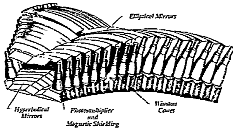
Figure 2-11. Cerenkov detector in CLAS. Here is shown a picture of its structure in each sector
