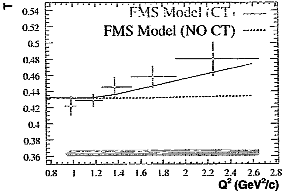
Figure 6-12. The Nuclear Transparency ratio for Iron and Deuterium targets with beam energy of 5\text{GeV} is plotted here as a function of Q^2 . Theoretical predictions with a model from L. Frankfurt, G.A. Miller, M. Strikman (FMS, see section 1.3.4 of this thesis) are also plotted to better interpret the data. The blue curve represents the theoretical prediction with a Glauber based model (NO CT). From this theory one is expected to see a more constant behavior with a variation in Q^2 . If one adds to this model the properties of Color Transparency one obtains a dependence on the Nuclear Transparency ratio respects to Q^2 (red curve). The data for Iron at 5\text{GeV} shows a consistent increase in Q^2 with a better statistical significant respect to the other configurations inspected in this experiment. This is due to the higher statistic available in this particular configuration. The difference respect to the expected behavior from a Glauber calculation is important. The data presents consistently higher values for the part with higher Q^2 respect to the one predicted by the FMS model. A \chi^2 study in this result rejects the Glauber model calculation with a confidence level of 94%.
