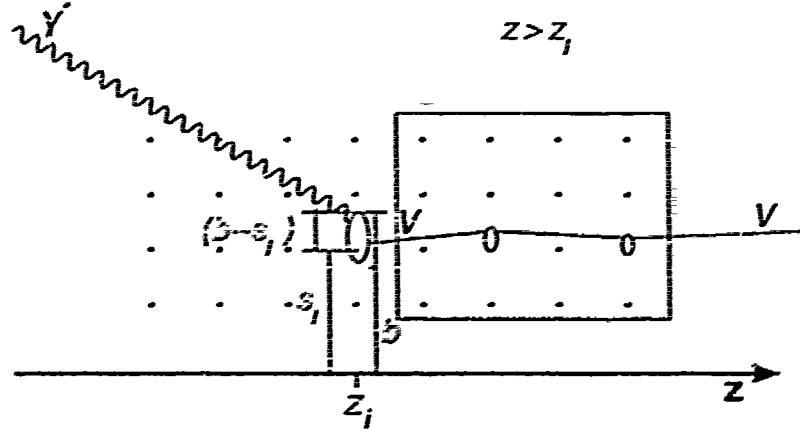
Figure 1.3. Schematic of the interaction in an atom using the Glauber approximation. On red are outlined the region where the nuclei will contribute with elastic scattering depending on their local impact parameter. \vec{b} will describe the transverse coordinate (respect to the symmetry axis z ) of the incoming \gamma^* . \vec{s}_j will describe the transverse coordinate of the nucleus j . (\vec{b} - \vec{s}_j) will describe the impact parameter of the \gamma^* respect to the nucleus j
