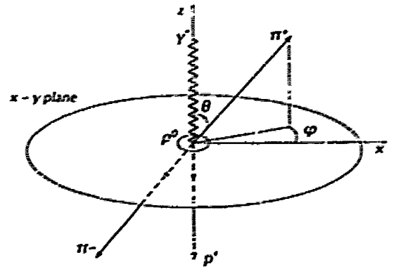
Figure 5-12: \rho^0 decay in the \rho^0 rest system.
