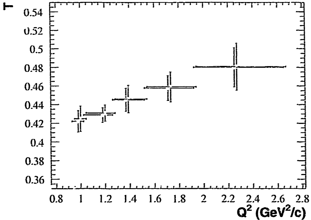
Figure 6-7. Comparison of Nuclear Transparency ratio for Iron data at 5GeV and determined with two different acceptance correction (see section 5.2 of this thesis). In green is shown the result obtained with a "bin by bin" acceptance correction. In red is shown the one obtained considering also the "bin migration" effect. The data is plotted with errors due to statistical and point to point systematical (added in quadrature). The colored bad in the bottom represents the systematical error identified before as "normalization" (see section 5.5 of this thesis). This last systematical error causes a common shift in all the point of the distribution, and does not contribute to the physical behavior of the Nuclear Transparency ratio (for this reason is not included with the other error).
