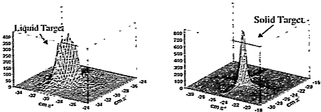
Figure 3-9. After we require that the event has an electron with vertex correspondent to one of the two targets, the selection of the target for z^+ and z^- from the same event results easier. In these plots are shown the vertices distribution for z^+ and z^- after we already have applied our cut for the electron track
