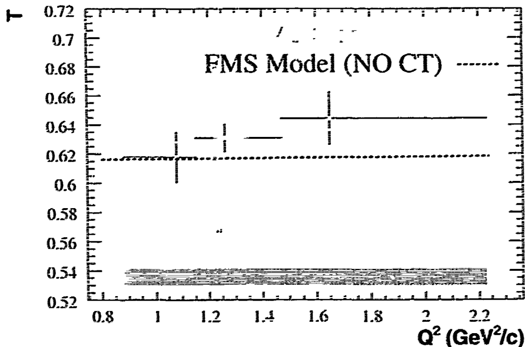
Figure 6-9. The Nuclear Transparency ratio for Carbon and Deuterium targets with beam energy of 5\text{GeV} is plotted here as a function of Q^2 . Theoretical provisions with a model from L. Frankfurt, G.A. Miller, M. Strikman (FMS, see section 1.3.1 of this thesis) are also plotted to better interpret the data. The blue curve represents the theoretical provision with a Glauber based model (NO CT). From this theory one is expected to see a more constant behavior with a variation in Q^2 . If one adds to this model the properties of Color Transparency one obtains a dependence on the Nuclear Transparency ratio respects to Q^2 (red curve). The data for Carbon at 5\text{GeV} shows an increase in Q^2 which cannot be interpret using a Glauber model. A \chi^2 study in this result rejects the Glauber model calculation with a confidence level of 81%.
