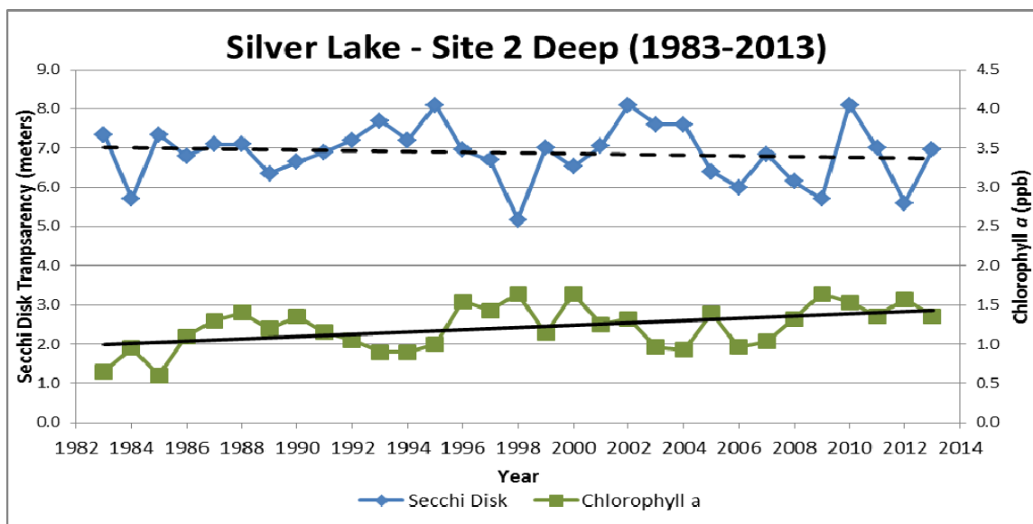
Figure 2. Changes in water clarity (Secchi disk depth) and chlorophyll a measured from 1983-2013 at Site 2 Deep. There has been a slight declining trend in water clarity since 1983, although not statistically significant (dashed line). Decreasing water clarity is a negative trend for lakes if caused by increased algae or polluted runoff. Algal growth has increased over the thirty one years of sampling and has been significant with time (chlorophyll; solid line).
