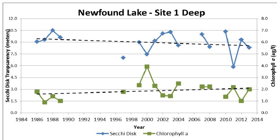
Figure 2. Changes in the Newfound Lake water clarity (secchi disk depth) and chlorophyll a concentrations measured between 1986 and 2013 at site 1 Deep. The long-term water clarity data indicate a trend of declining water clarity (dashed line). The long-term algal growth (chlorophyll a ) data indicate a trend of increasing concentrations (dashed line). Neither the long-term water clarity nor the long-term chlorophyll a trend is statistically significant.
