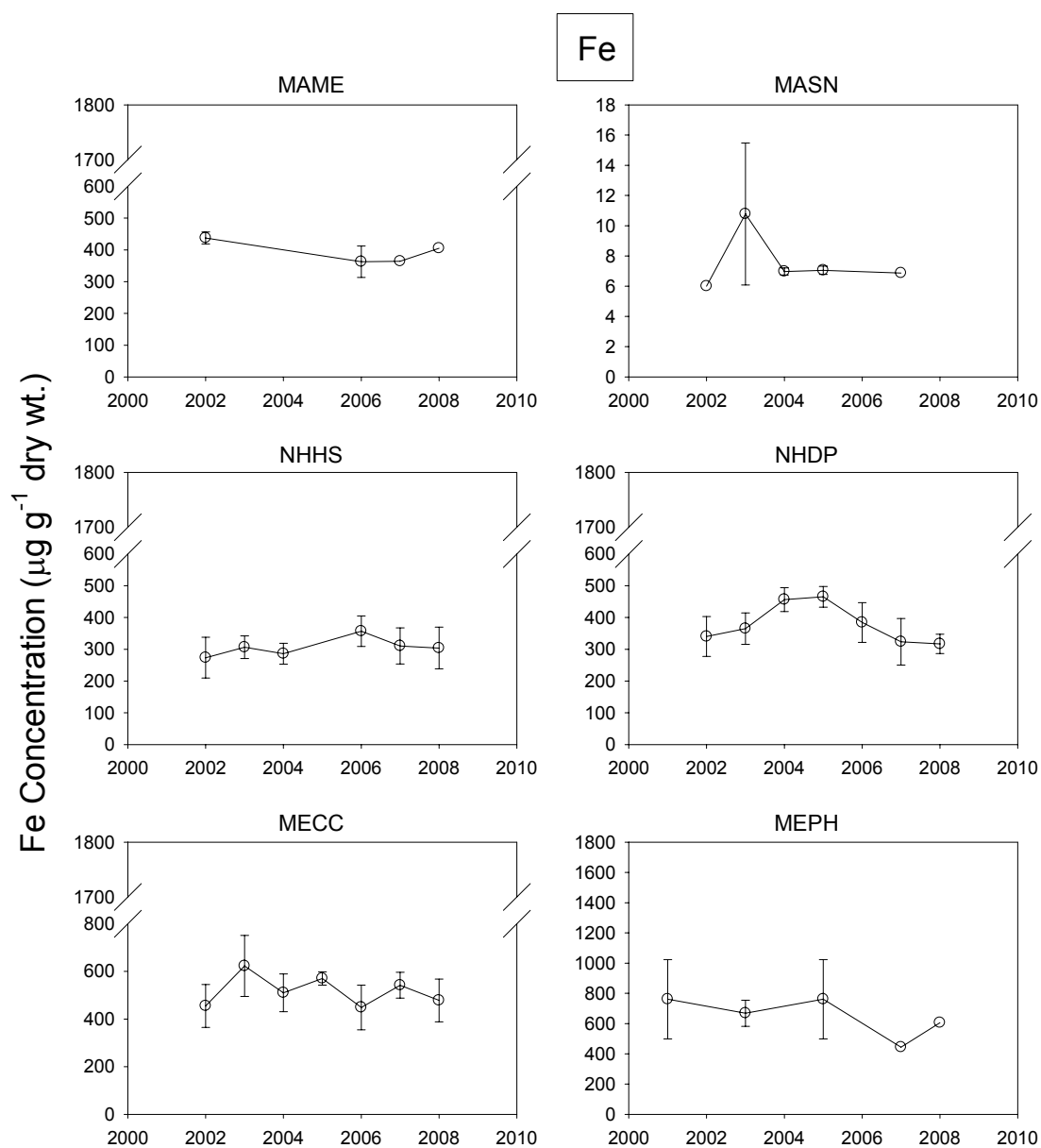
Figure 20. Distribution of iron tissue concentrations in µg/g dry weight (arithmetic mean \pm standard deviation) in mussels at Gulfwatch trend sites in 2001-2008. For 2007 and 2008 there are only single site composite values except for stations NHDP, NHHS and MECC.
