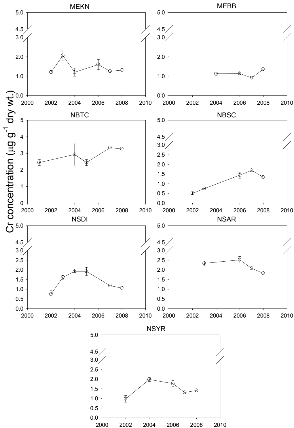
Figure 18 (cont'd). Distribution of chromium tissue concentrations in \mu\text{g/g} dry weight (arithmetic mean \pm standard deviation) in mussels at Gulfwatch trend sites in 2001-2008. For 2007 and 2008 there are only single site composite values except for stations NHDP, NHHS and MECC.
