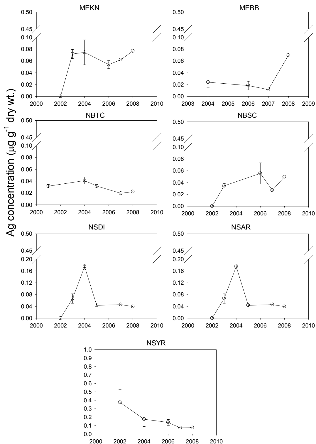
Figure 16 (cont'd). Distribution of silver tissue concentrations in \mu\text{g/g} dry weight (arithmetic mean \pm standard deviation) in mussels at Gulfwatch trend sites in 2001-2008. For 2007 and 2008 there are only single site composite values except for stations NHBC, NHDP, NHHS and MECC.
