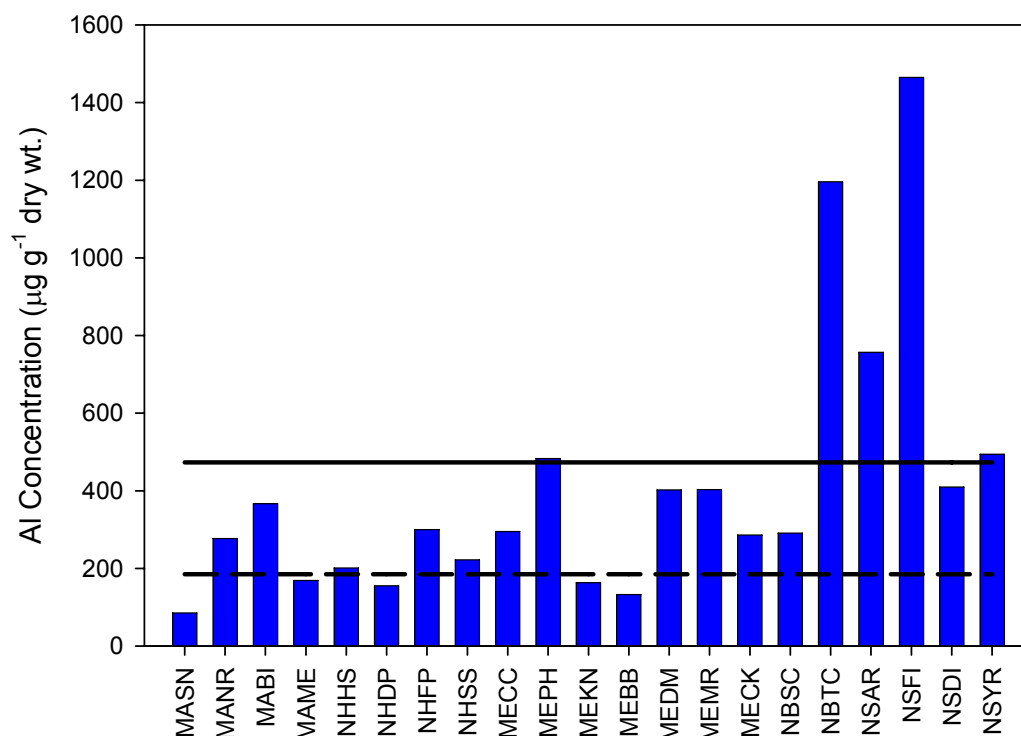
Figure 7. Distribution of aluminum tissue concentrations in mussel sample site composites (one per site) at Gulfwatch sites in 2008. Dashed line = 2008 Mussel Watch National median; Solid line = 2008 Mussel Watch 85 th percentile.
