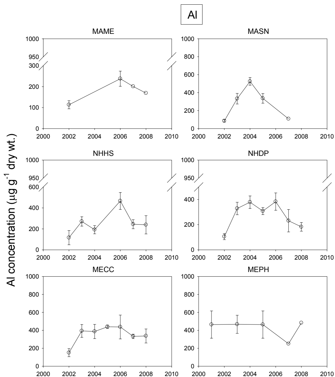
Figure 21. Distribution of aluminum tissue concentrations in \mu\text{g/g} dry weight (arithmetic mean \pm standard deviation) in mussels at Gulfwatch trend sites in 2001-2008. For 2007 and 2008 there are only single site composite values except for stations NHDP, NHHS and MECC.
