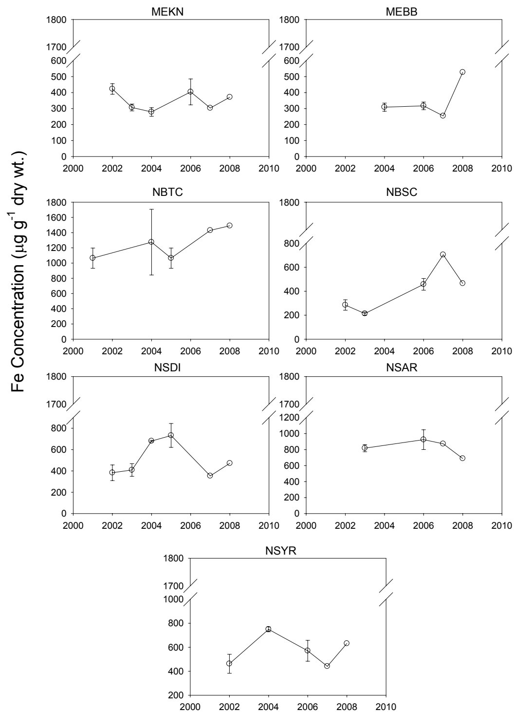
Figure 20 (cont'd). Distribution of iron tissue concentrations in \mu\text{g/g} dry weight (arithmetic mean \pm standard deviation) in mussels at Gulfwatch trend sites in 2001-2008. For 2007 and 2008 there are only single site composite values except for stations NHDP, NHHS and MECC.
