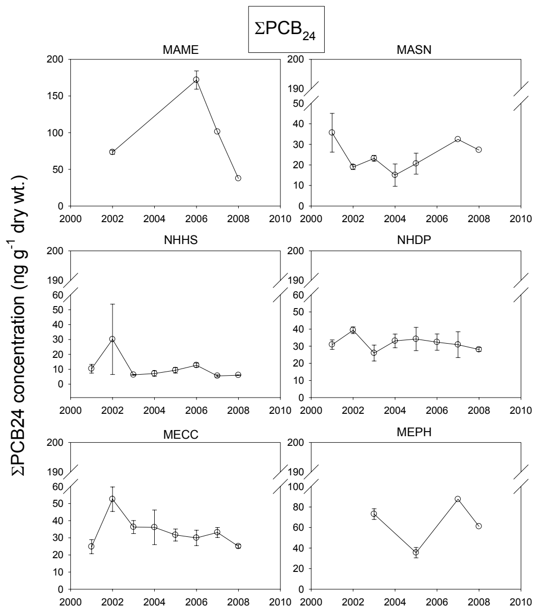
Figure 27. Distribution of the sum of 24 PCB congeners in \text{ng/g} dry weight (arithmetic mean \pm standard deviation) in mussels at Gulfwatch trend sites in 2001-2008. For 2007 and 2008 there are only single site composite values except for stations NHDP, NHHS and MECC.
