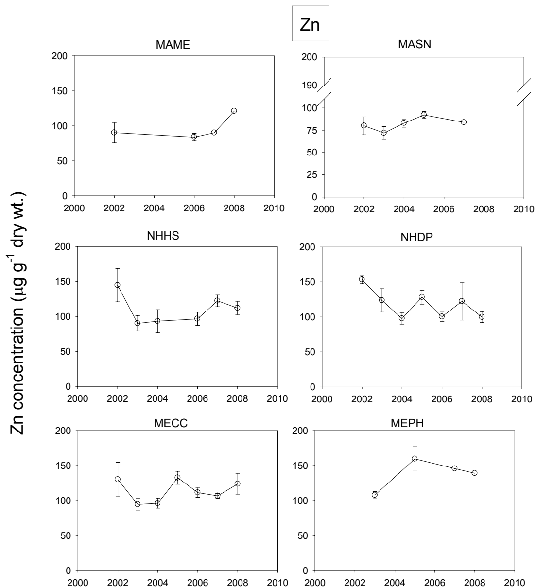
Figure 24. Distribution of zinc tissue concentrations in \mu\text{g/g} dry weight (arithmetic mean \pm standard deviation) in mussels at Gulfwatch trend sites in 2001-2008. For 2007 and 2008 there are only single site composite values except for stations NHDP, NHHS and MECC.
