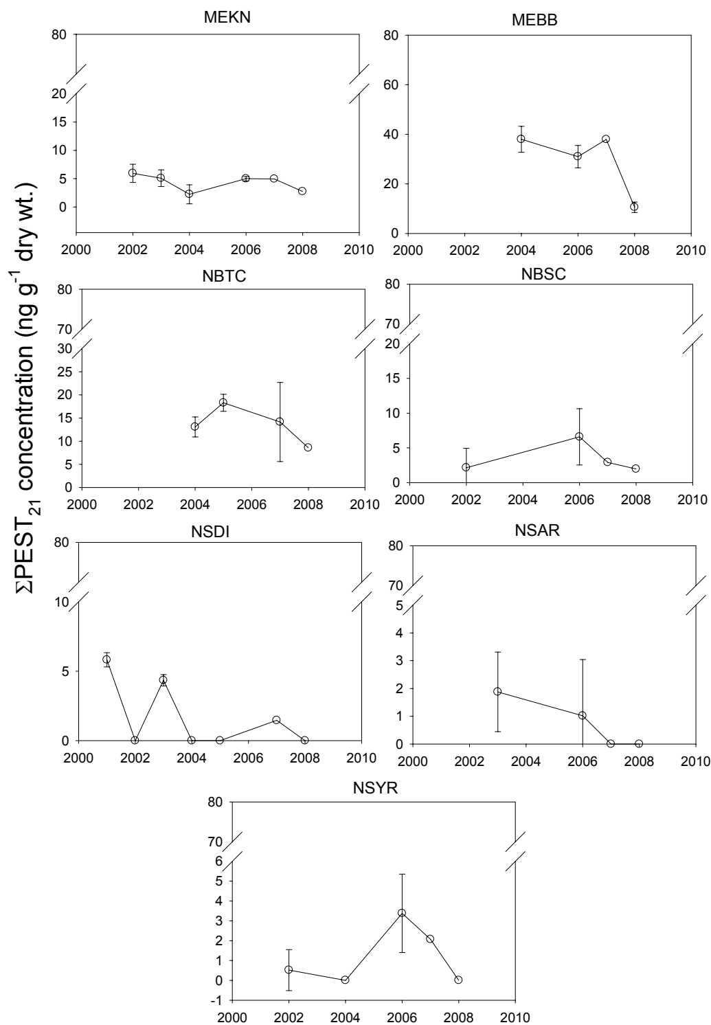
Figure 28 (cont'd). Distribution of the sum of 21 chlorinated pesticide compounds in ng/g dry weight (arithmetic mean \pm standard deviation) in mussels at Gulfwatch trend sites in 2001-2008. For 2007 and 2008 there are only single site composite values except for stations NHDP, NHHS and MECC.
