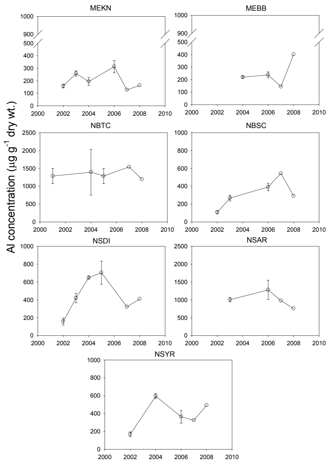
Figure 21 (cont'd). Distribution of aluminum tissue concentrations in \mu\text{g/g} dry weight (arithmetic mean \pm standard deviation) in mussels at Gulfwatch trend sites in 2001-2008. For 2007 and 2008 there are only single site composite values except for stations NHDP, NHHS and MECC.
