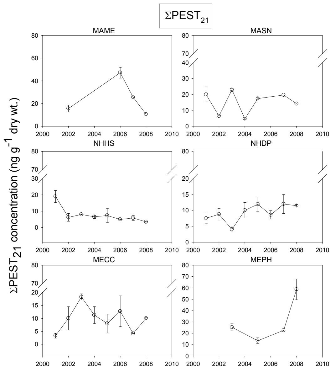
Figure 28. Distribution of the sum of 21 chlorinated pesticide compounds in \text{ng/g} dry weight (arithmetic mean \pm standard deviation) in mussels at Gulfwatch trend sites in 2001-2008. For 2007 and 2008 there are only single site composite values except for stations NHDP, NHHS and MECC.
