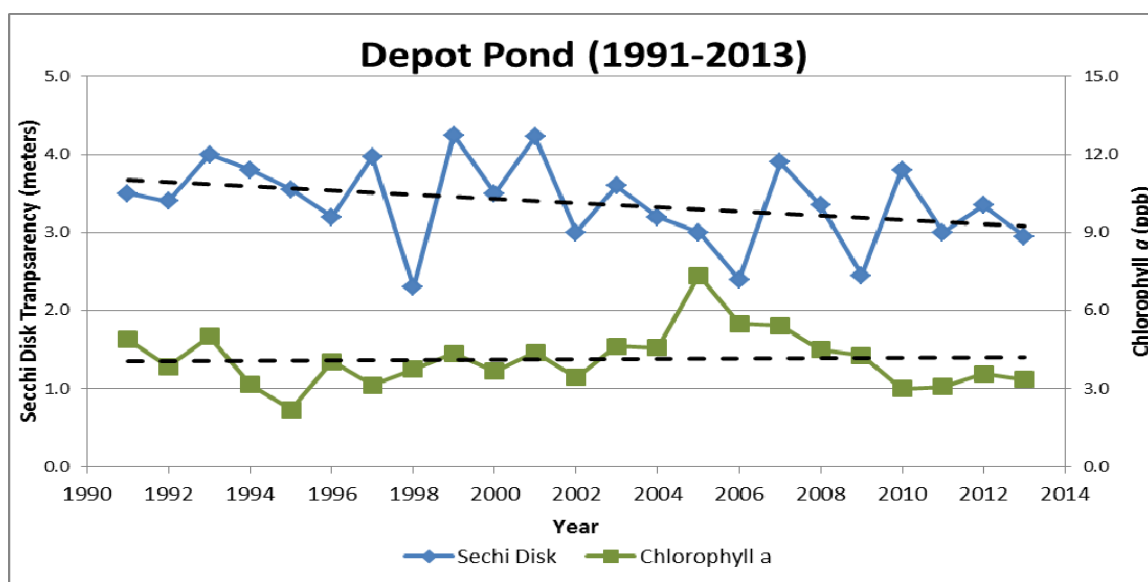
Figure 2. Changes in water clarity (Secchi disk depth) and chlorophyll a measured between 1991 and 2013 in Depot Pond. The long-term water clarity data indicate a trend of decreasing water clarity (dashed line). The algal growth (chlorophyll a ) data indicate a relatively stable long-term trend (dashed line). Neither the Secchi Disk transparency nor the chlorophyll a trend is statistically significant.
