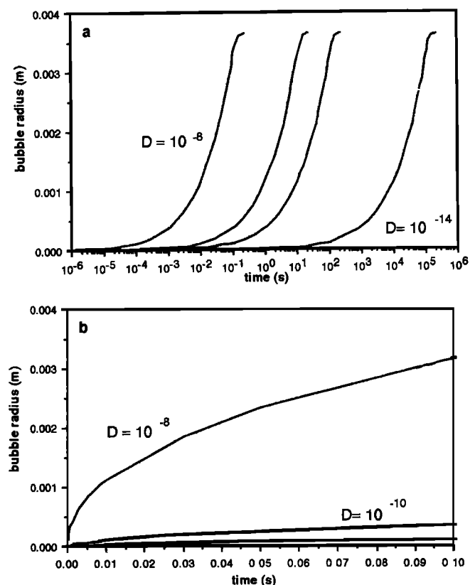
Figure 2. Effect of diffusivity for negligible viscosity and surface tension. (a) In model runs with all parameters the same except for diffusivity, it was found that without the inhibiting effects of viscosity and surface tension, the family of growth curves for rhyolite are self-similar, as in the case for basalt. This indicates that rapid growth rates (even with very high diffusivities) are unimpeded under these conditions. (b) When plotted with linear timescale, it is evident that there is no time delay (accelerating growth phase) even for the highest diffusivity ( 10^{-8} m ^2 /s). Growth rate was clearly impeded in model runs with normal rhyolitic viscosity and surface tension [ Prousevitich et al. , 1993, Figure 15]. This is one illustration of the importance of viscosity and surface tension to bubble growth. All curves had the following values for parameters: initial bubble radius, 4.4 \times 10^{-7} m ( 0.44 \mu m); viscosity, 10^{-4} Pa s; surface tension, 10^{-6} J/m ^2 .
