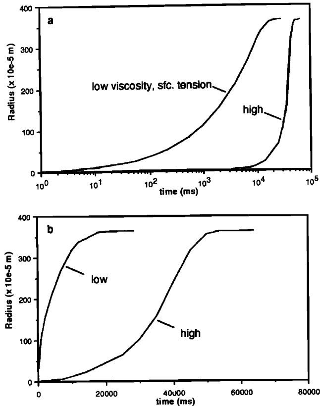
Figure 1. Effect of viscosity and surface tension on early bubble growth. The "high" case has normal magmatic viscosity and surface tension of 10^6 Pa s and 0.32 J/m ^2 , respectively. The "low" case has 10^{-5} Pa s and 10^{-6} J/m ^2 , respectively (essentially zero). (a) When plotted on a logarithmic timescale, the curves show a clear difference in growth pattern. (b) A linear time scale highlights the absence of an "accelerating growth phase" for unrealistically low viscosity and surface tension but its presence for normal conditions. This suggests that the accelerating growth phase is not dependent upon geometry but is controlled by viscosity and/or surface tension. Both curves had the following values for relevant parameters: Initial bubble radius, 10^{-5} m; diffusivity, 10^{-10} m ^2 /s. All curves in this and following figures have the following: ambient Pressure, 0.1 Mpa; initial dissolved volatile concentration, 0.5%.
