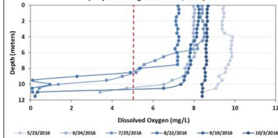
Figure 6. Lovell Lake, Site 2 South - Dissolved Oxygen Profiles (May 23 through October 3, 2016)
