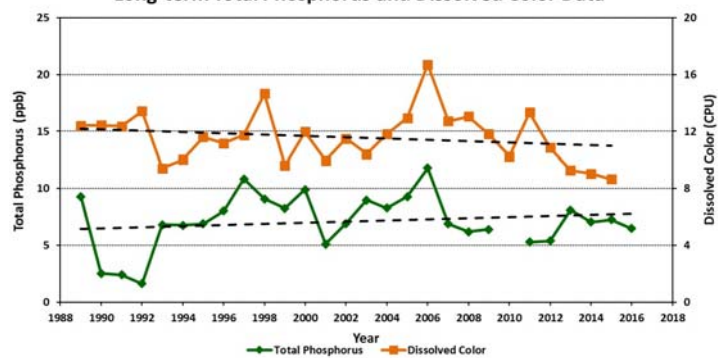
Figure 5. Lovell Lake - Site 2 South (1989-2016) Long-term Total Phosphorus and Dissolved Color Data
