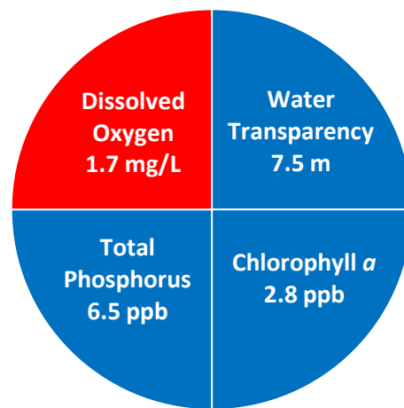
Figure 1. Lovell Lake Water Quality (2016)
