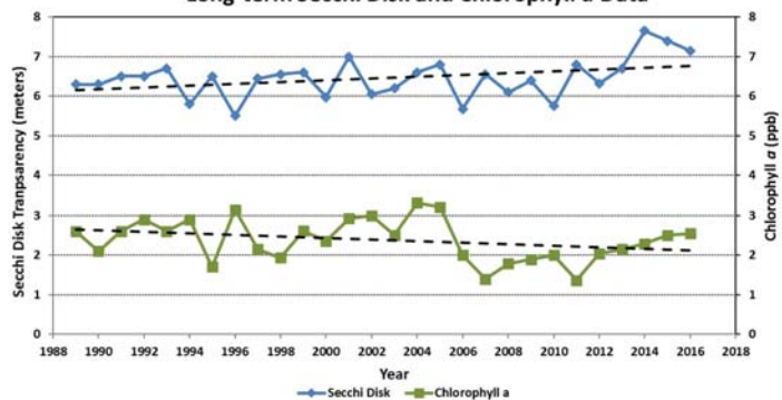
Figure 4. Lovell Lake - Site 2 South (1989-2016) Long-term Secchi Disk and Chlorophyll a Data
