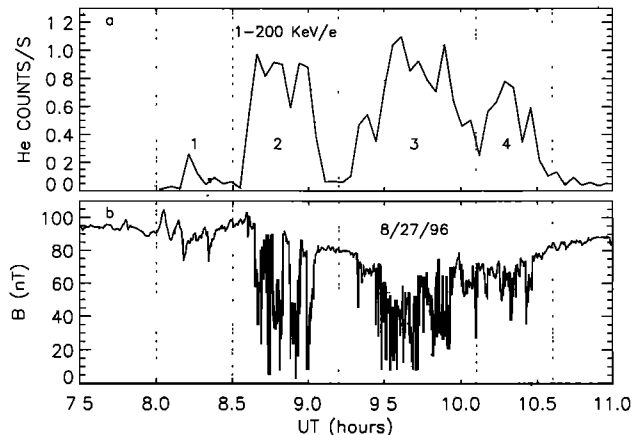
Figure 1. An example of the CEP events on August 27, 1996. (a) The 1-200 KeV/e helium counting rate versus time, (b) the corresponding variation of the local geomagnetic field, where the vertical dashed lines mark the four different regions in the events.
