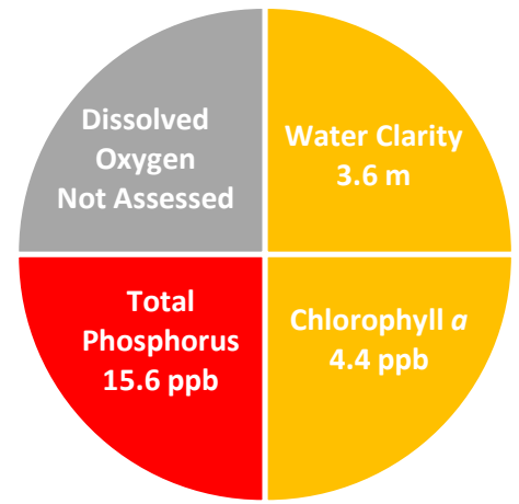
Figure 1. Naticook Lake Water Quality (2017)
