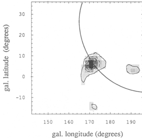
Figure 6. Maximum entropy skymap of the GRB 910503 burst region. The contours are given in relative flux units. The triangulation circle derived from COMPTEL/Ulysses arrival time analysis is shown.
