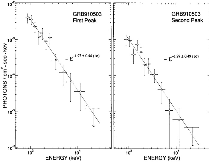
Figure 4. Best fit telescope event spectra for first pulse (25454 s - 25464 s) and second pulse (25500 s - 25510 s) of GRB 910503.
