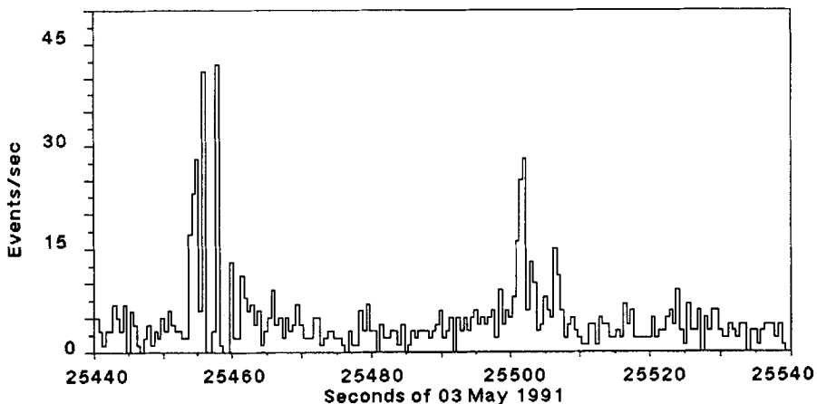
Figure 2. GRB 910503: Lightcurve from COMPTEL imaging events. Data contain raw events without application of any selection criteria.
