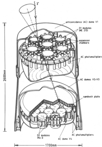
Figure 1. Schematic view of COMPTEL.
