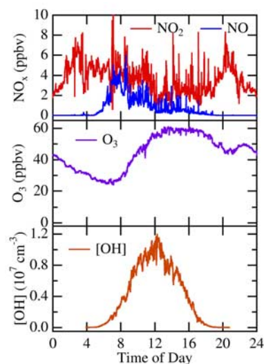
Figure 4. Diurnal averaged mixing ratios of NO x (NO and NO 2 ) (upper) and O 3 (middle). The spikes in NO x are due to ship plumes, which have been filtered from the data at night (60 data points removed out of more than 15,000 in the average). The lower panel shows the averaged calculated OH concentration.
