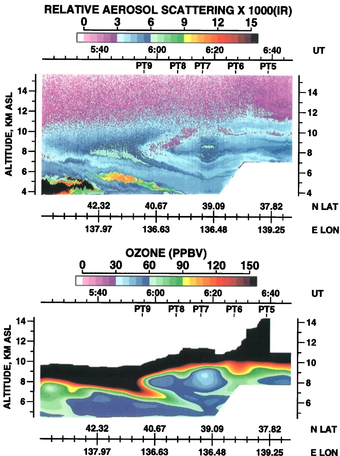
Plate 1. Zenith profiles of \text{O}_3 and aerosol scattering from the UV-DIAL instrument. These data were collected during the 3.4 km leg of the vertical wall, looking upward at the air masses the DC-8 had earlier flown through. A tropopause fold is clearly outlined in both sets of data.
