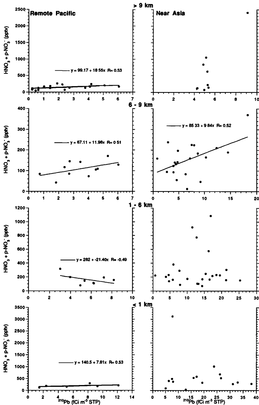
Figure 5. Scatterplots of ^{210}\text{Pb} versus \text{HNO}_3 plus \text{p-NO}_3 in the eight data bins. Correlation coefficients for all bins without regression lines plotted (and more than three sample pairs) were \leq 0.30 .
