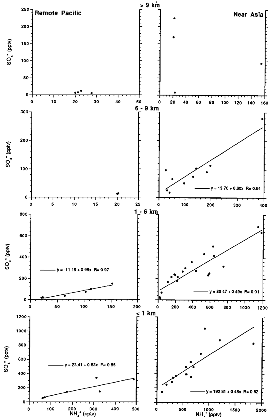
Figure 3. Scatterplots of \text{SO}_4^{2-} versus \text{NH}_4^+ in the eight data bins. Correlation coefficients for all bins without regression lines plotted (and more than three sample pairs) were \leq 0.25 .
