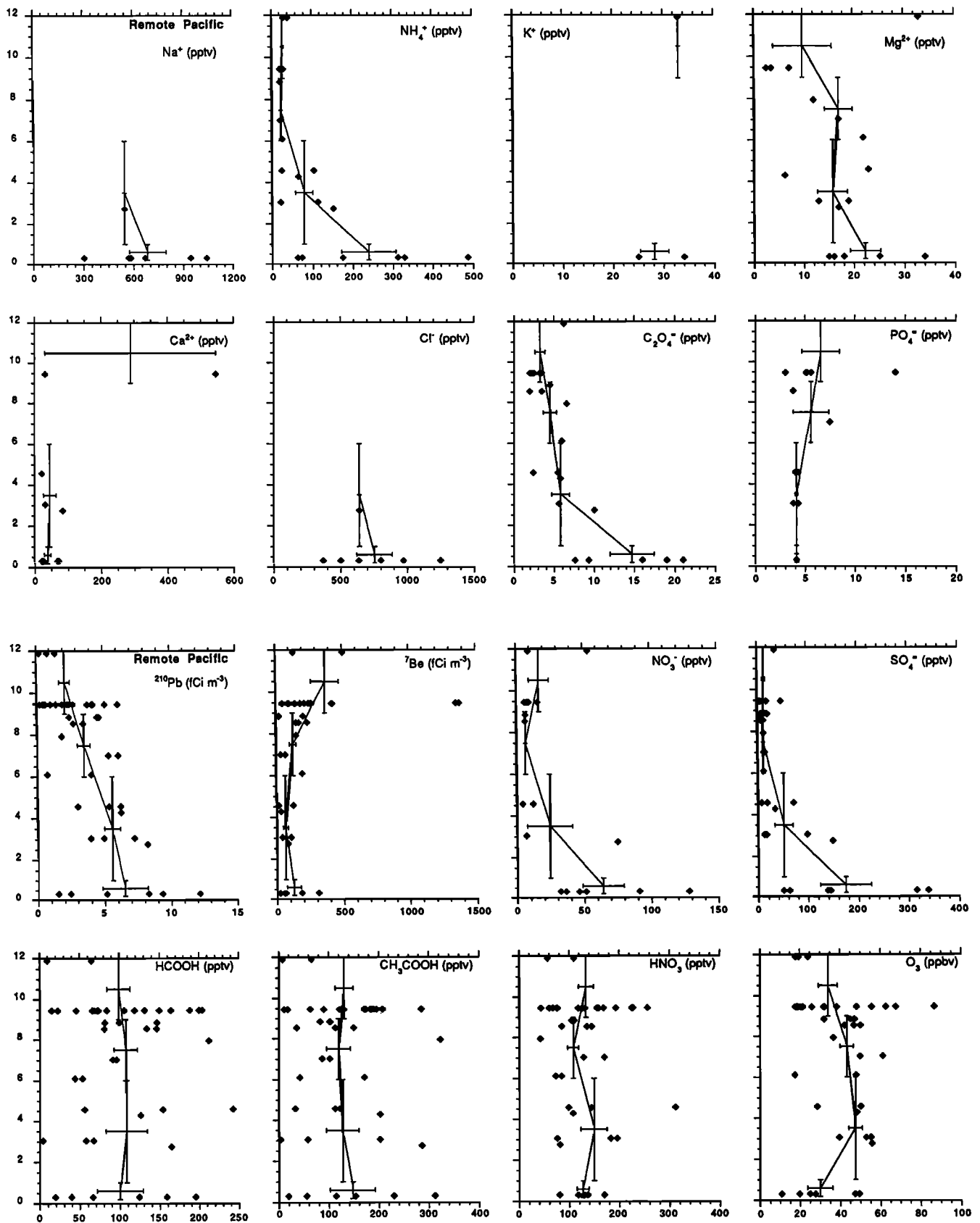
Figure 1. Mean concentrations of soluble aerosol-associated species, soluble acidic gases and ozone versus altitude (km) over the western Pacific during PEM-West B. All samples with concentrations above detection limits in the "remote Pacific" and "near-Asia" regions are plotted. The horizontal arms of the crosses represent the standard error of the mean for each species in the eight region/altitude bins presented in Table 1, while the altitude range is encompassed by the vertical arms.
