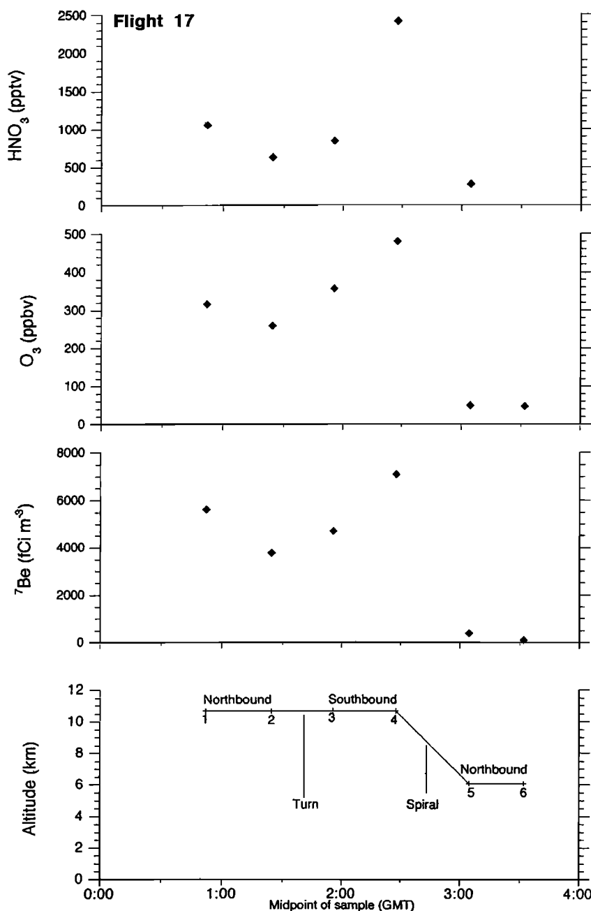
Figure 9. Mean concentrations of \text{HNO}_3 , \text{O}_3 and ^7\text{Be} in the first six aerosol sampling intervals of flight 17. As depicted in the lower panel, the first four aerosol samples were all collected during the 10.7 km leg of the wall, with five and six from the 6.1 km leg.
