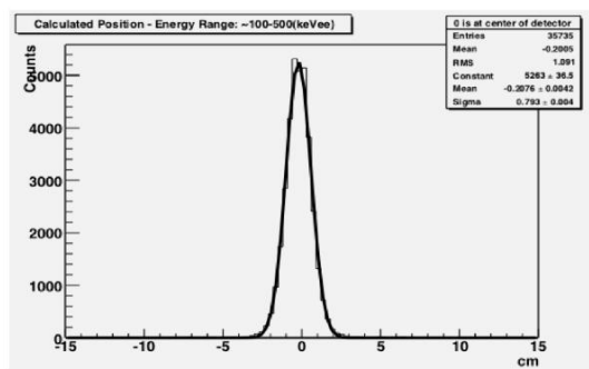
Fig. 5. A measured 0.7 cm position resolution in a rod.
