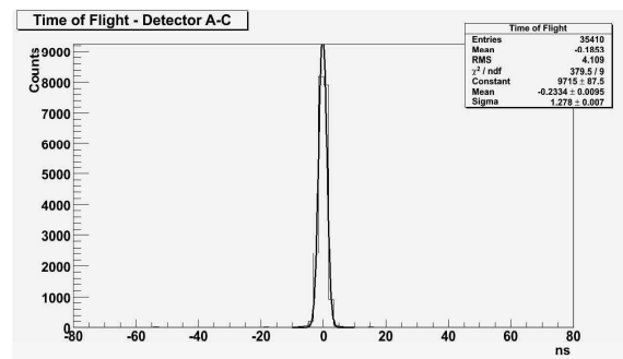
Fig. 6. The ToF resolution of 1.3 ns.
