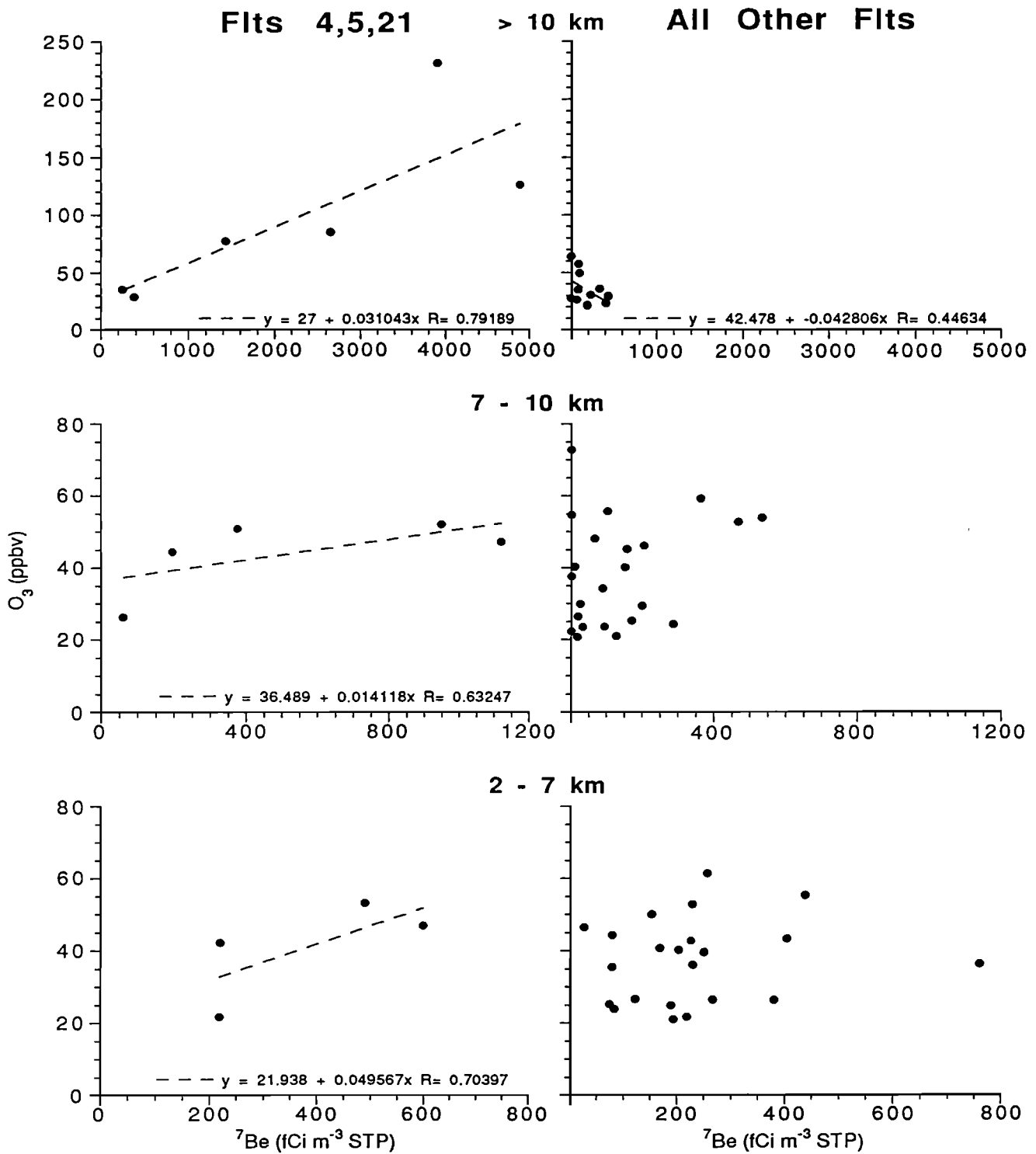
Figure 4. Scatterplots of O 3 against 7 Be in the free troposphere. The three transit flights (4, 5, and 21) were flown between California and Alaska, Alaska and Japan, and from Hawaii to California. All remaining flights over the western Pacific are compared to these three.
