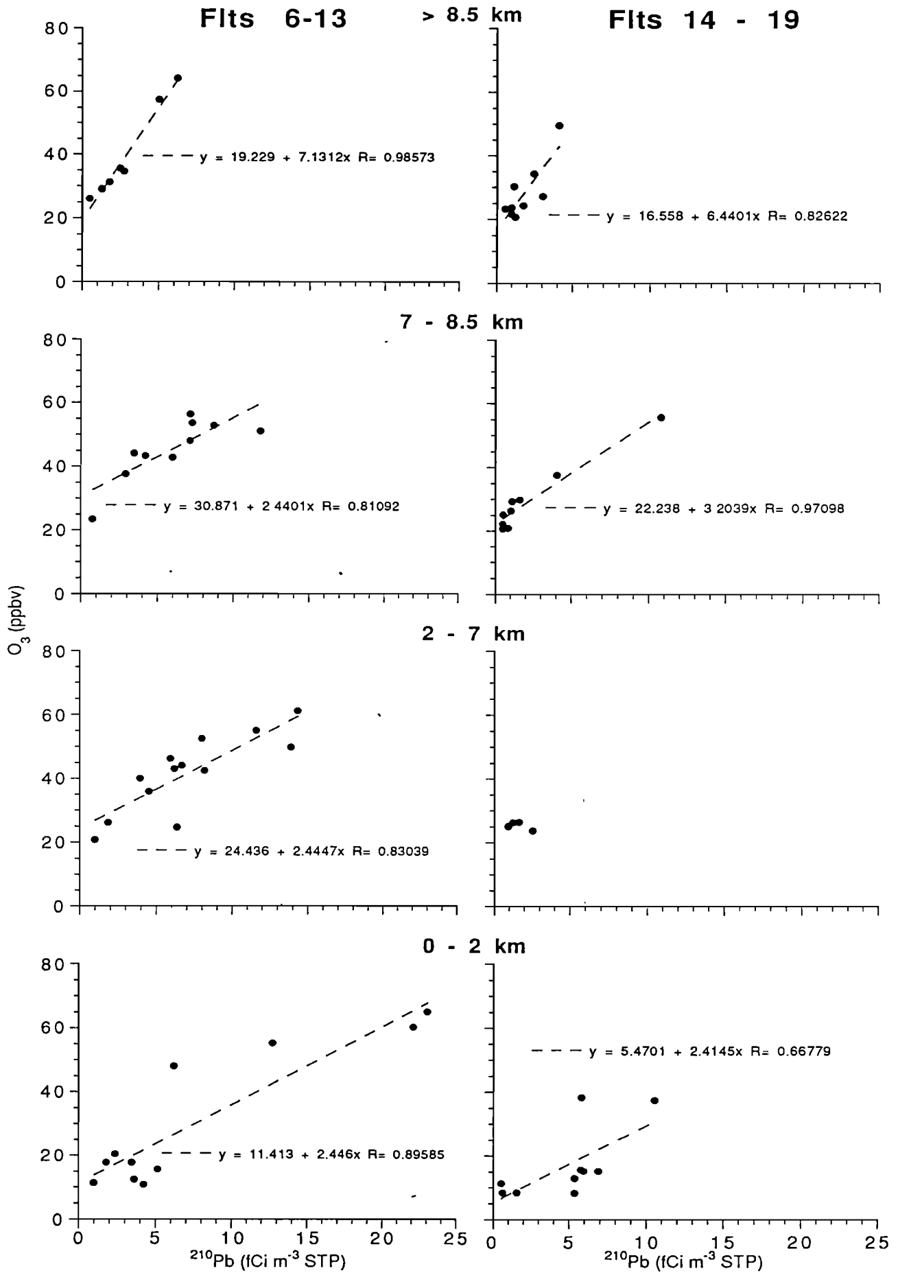
Figure 3. Scatterplots of O 3 against 210 Pb for the eight location/altitude bins depicted in Figure 1.
