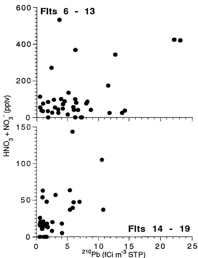
Figure 5. Scatterplots of atmospheric nitrate (aerosol NO 3 - plus HNO 3 ) against 210 Pb. Separate plots are shown for the samples collected near Asia and those from the remote western Pacific.
