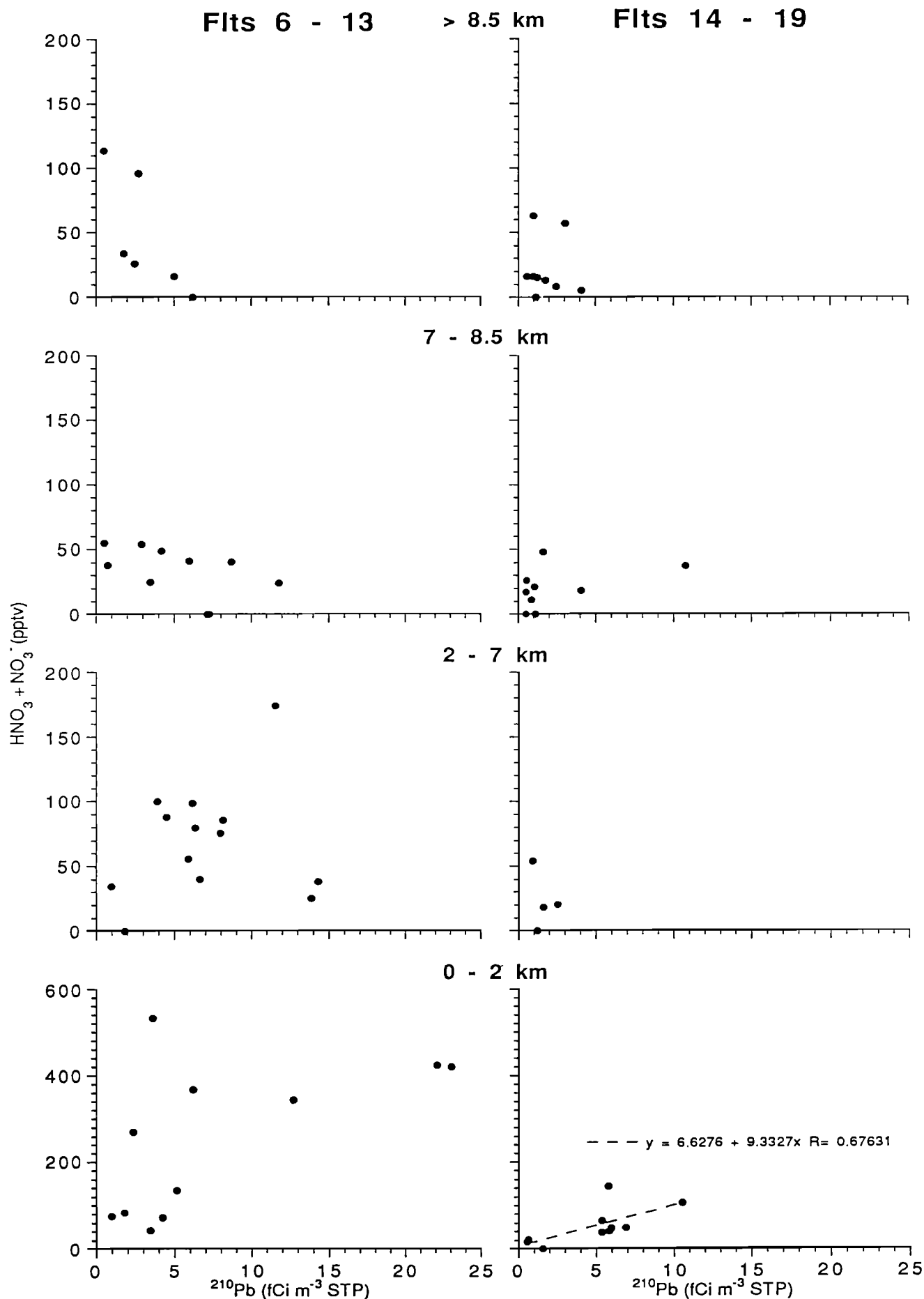
Figure 7. Scatterplots of atmospheric nitrate (NO 3 - plus HNO 3 ) against 210 Pb for the eight location/altitude bins depicted in Figure 6.
