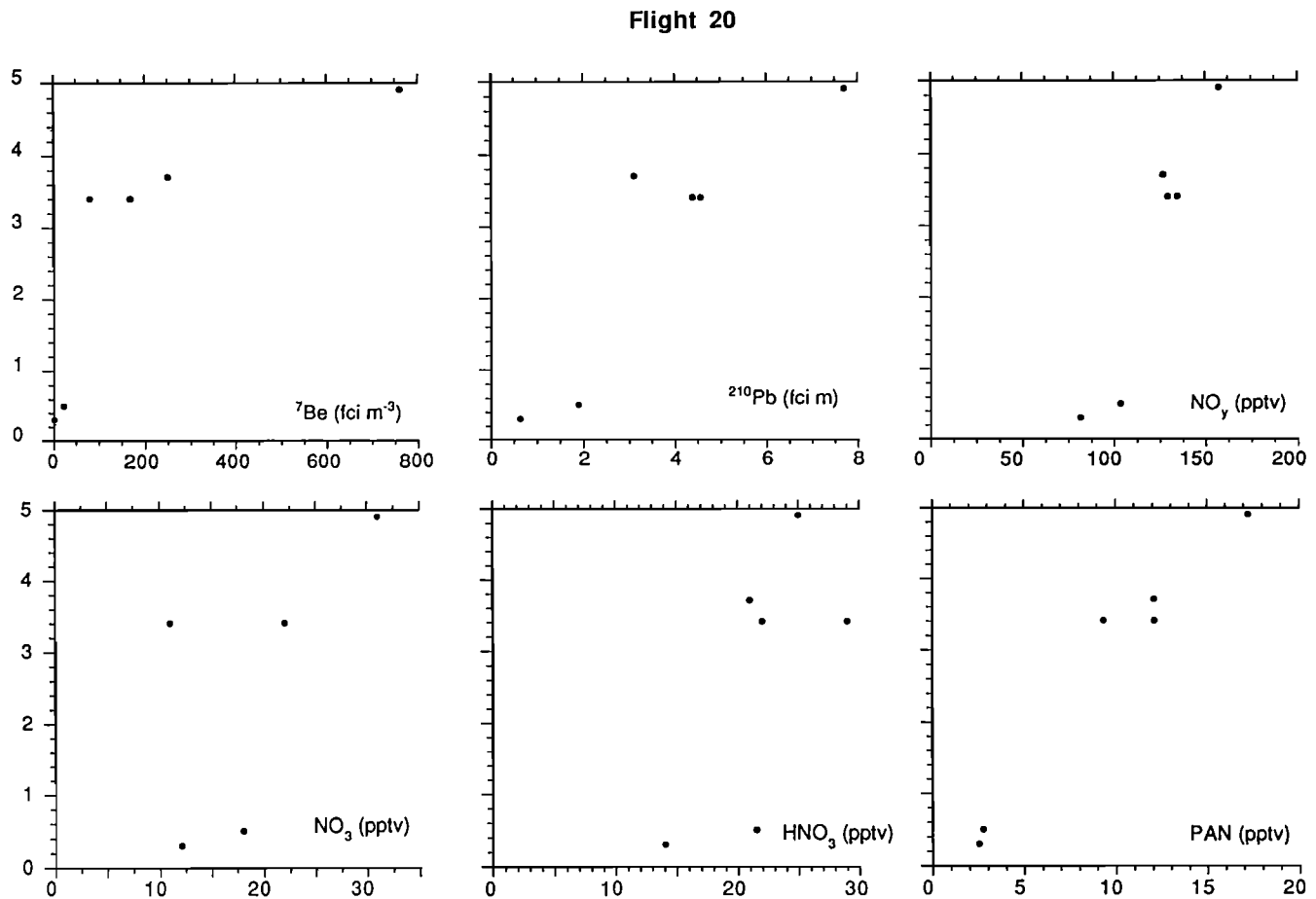
Figure 9. Altitude distributions of ^7\text{Be} , ^{210}\text{Pb} , \text{NO}_3^- , \text{HNO}_3 , PAN, and \text{NO}_y on flight 20, the Mauna Loa flyby.
