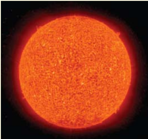
An image of a “quiet” Sun taken by STEREO’s Sun Earth Connection Coronal and Heliospheric Investigation (SECCHI) on February 21, 2009. Like the Sun images on page 1, this was taken in extreme ultraviolet light but at a different wavelength.
