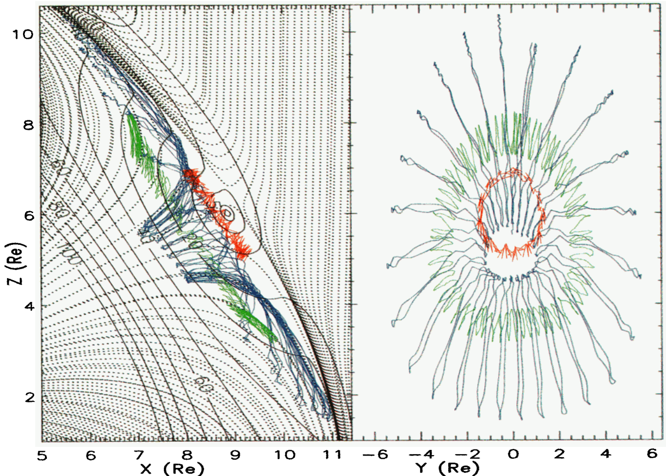
Figure 2. Trajectories of trapped 1 MeV electrons in the the Earth's outer cusp, projected into the GSM X-Z and Y-Z planes. Dashed lines are field lines from the T96 magnetic field model (Dipole: June 21, 1996, 1300UT; Solar Wind: +10nT Bz, 1/cm 3 , and 1000km/s V_{SW} ). Black lines are contours of |B| in nT. Green, blue and red trajectories correspond to the 1,3,4 entries of Table 1.
