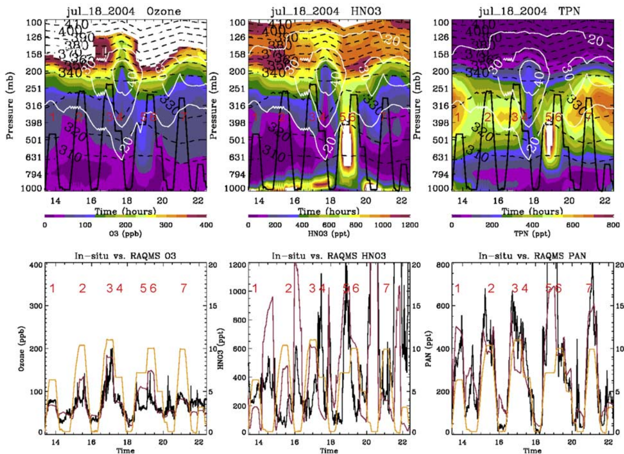
Figure 3a. (top) Curtains of RAQMS ozone, HNO 3 , and TPN along the DC8 flight track for 18 July 18. Isotachs (white), isentropes (black dashed) and DC8 flight profile (black) are also shown. Upper level FLs are numbered. (bottom) Corresponding time series of observed (black) and RAQMS (red) flight track data. Flight track altitude (km) is shown in orange, with axis marked at right.
