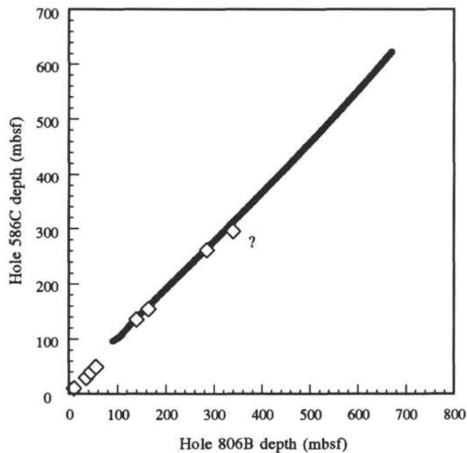
Figure 8. Stratigraphic correlation between Holes 806B and 586C, showing the inverse signal correlation map (solid line) compared to the nannofossil biostratigraphic events identified from the detailed post-cruise analysis (Takayama and Backman, this volume).
